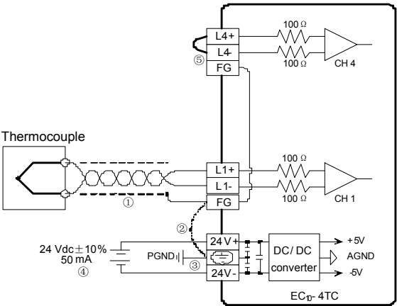
Figure 1-4 Wiring of EC10-4TC user port
